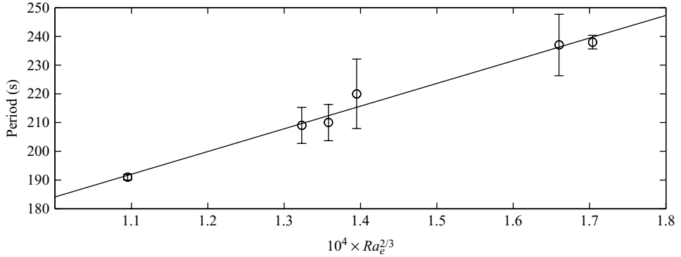
FIGURE 6. A comparison of the estimated periods for thermal formation and Howard's theory assuming heat transfer is independent of the layer depth.
